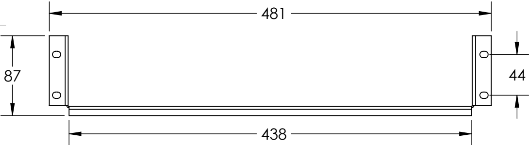
Vista frontal
